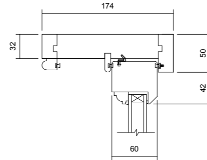
05 Head Detail 1 : 5
