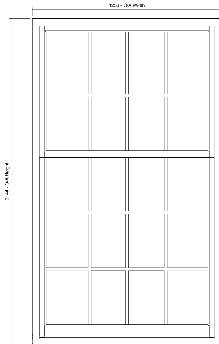
02 Front View 1 : 15
