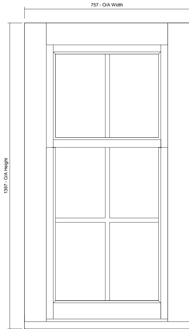
02 Front View 1 : 10
