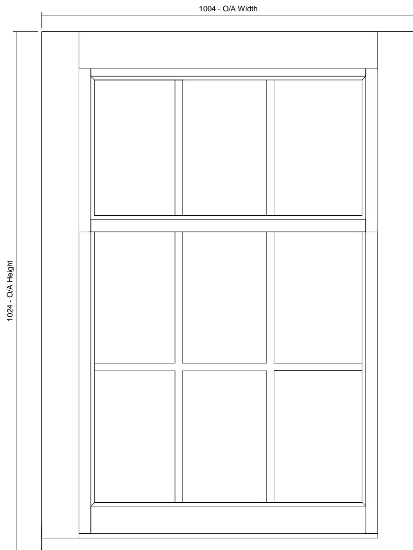
02 Front View 1 : 10
