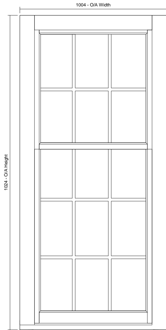
02 Front View 1 : 15
