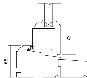
07 Cill Detail 1 : 5
