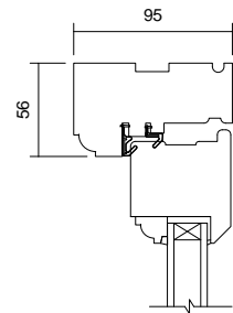
05 Head Detail 1 : 5
