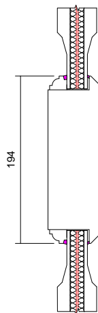
07 Mid Rail Detail 1 : 6
