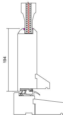
08 Threshold Detail 1 : 6
