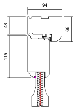
06 Head Detail 1 : 6
