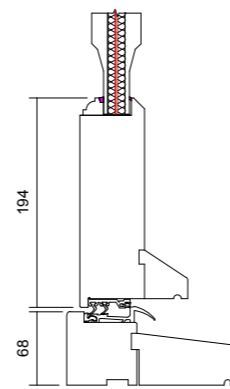
09 Threshold Detail 1 : 7
