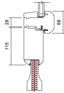
06 Top Rail & Transom Detail 1 : 7
