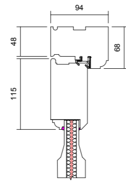
06 Head Detail 1 : 6
