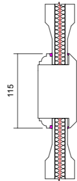
07 Frieze Rail Detail 1 : 6
