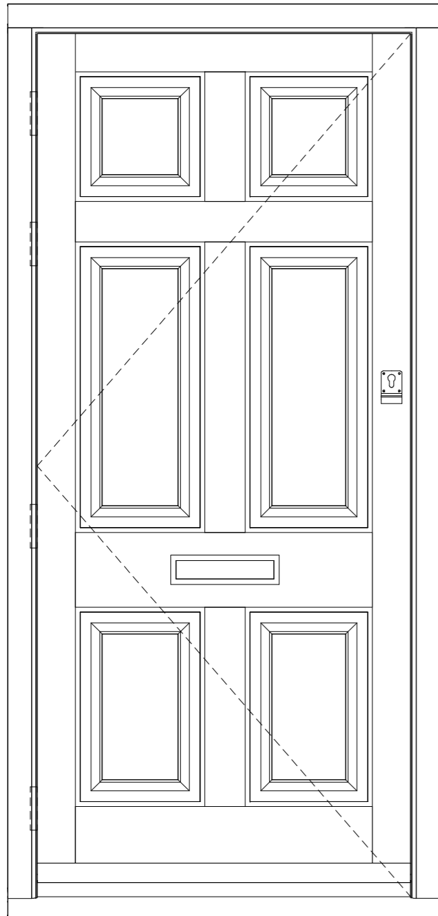
02 Front View 1 : 12
