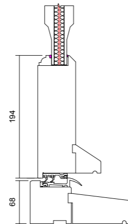
09 Threshold Detail 1 : 6
