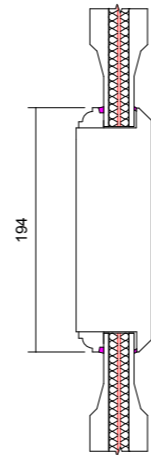
08 Mid Rail Detail 1 : 6
