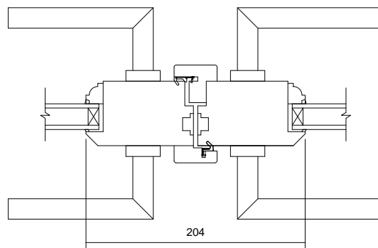
05 Meeting Stile 1 : 5
