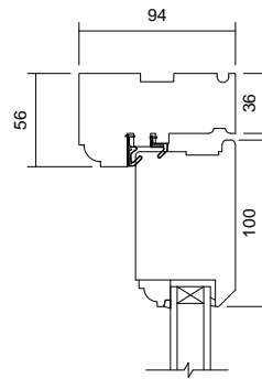
06 Head Detail 1 : 5
