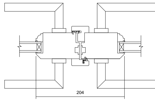
05 Meeting Stile 1 : 5
