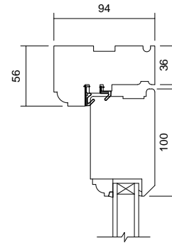
06 Head Detail 1 : 5
