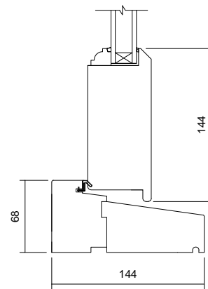
08 Threshold Detail 1 : 5
