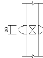
06 Glazing Bar Detail 1 : 5
