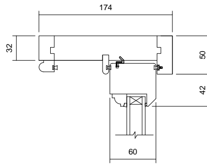
04 Head Detail 1 : 5
