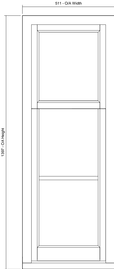
02 Front View 1 : 10
