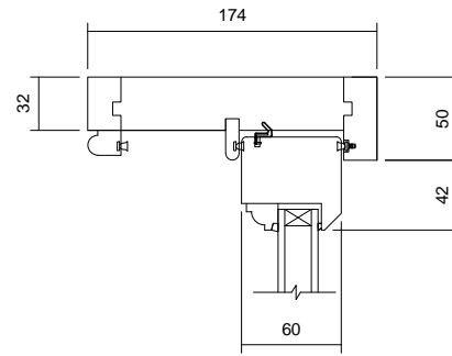
04 Head Detail 1 : 5
