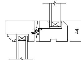
05 Meeting Rail Detail 1 : 5
