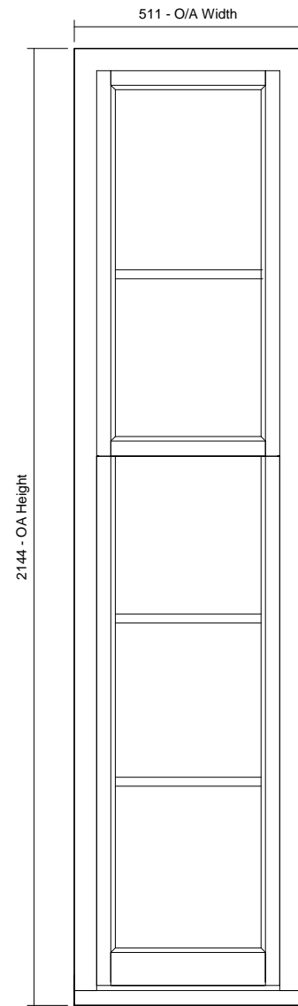
02 Front View 1 : 15
