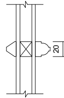
06 Glazing Bar Detail 1 : 5
