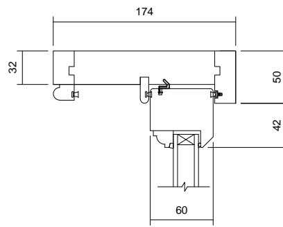
05 Head Detail 1 : 5
