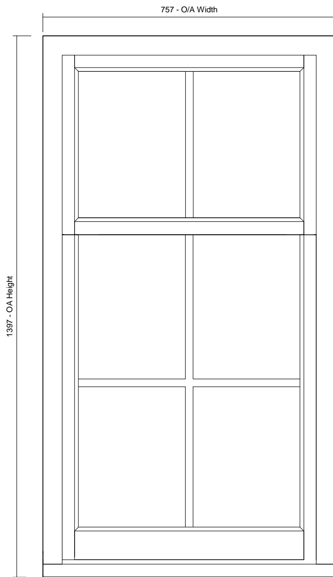
02 Front View 1 : 10
