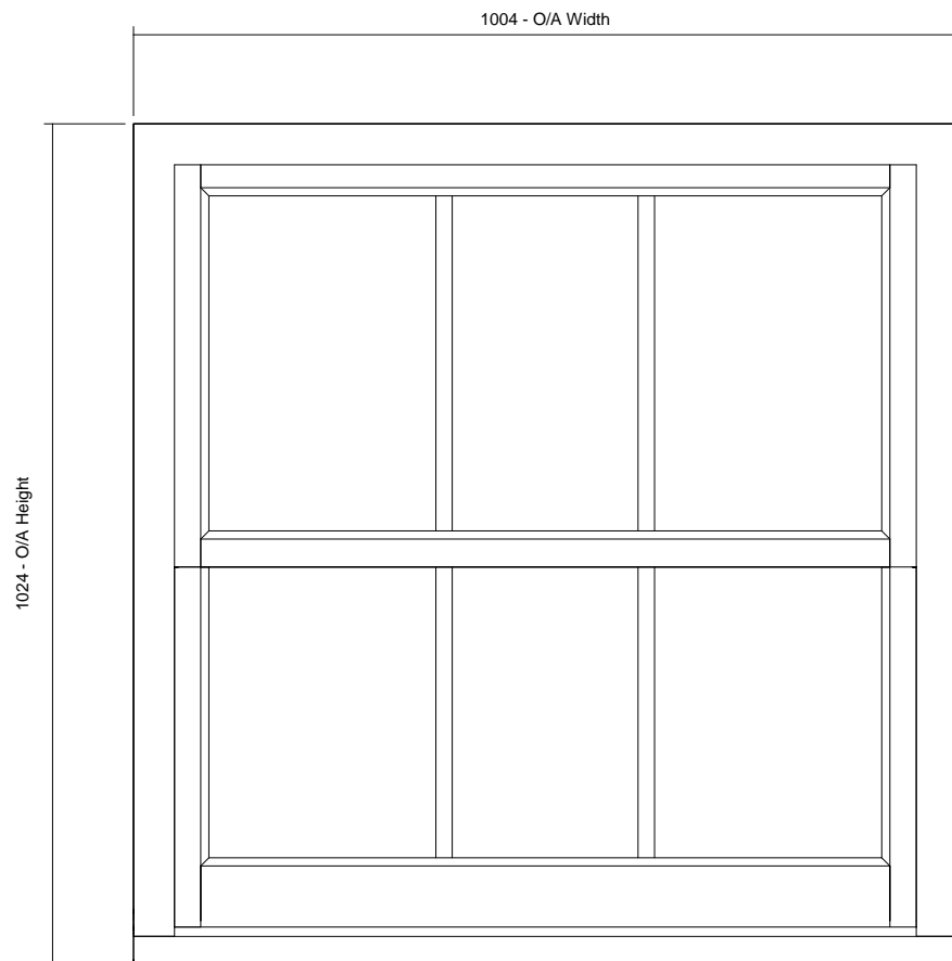
02 Front View 1 : 10
