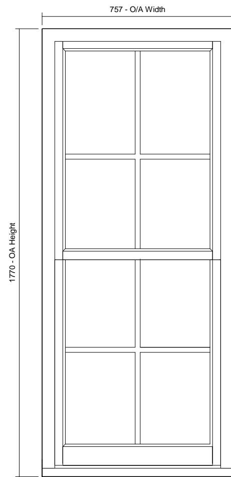
02 Front View 1 : 15
