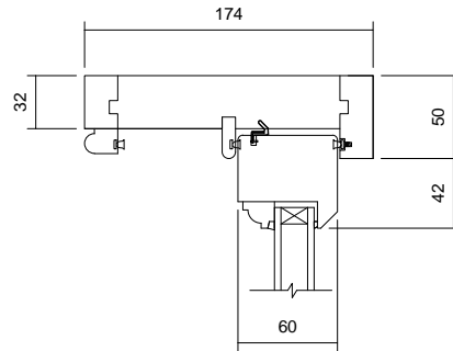
05 Head Detail 1 : 5
