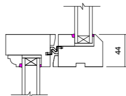
07 Meeting Rail Detail 1 : 5
