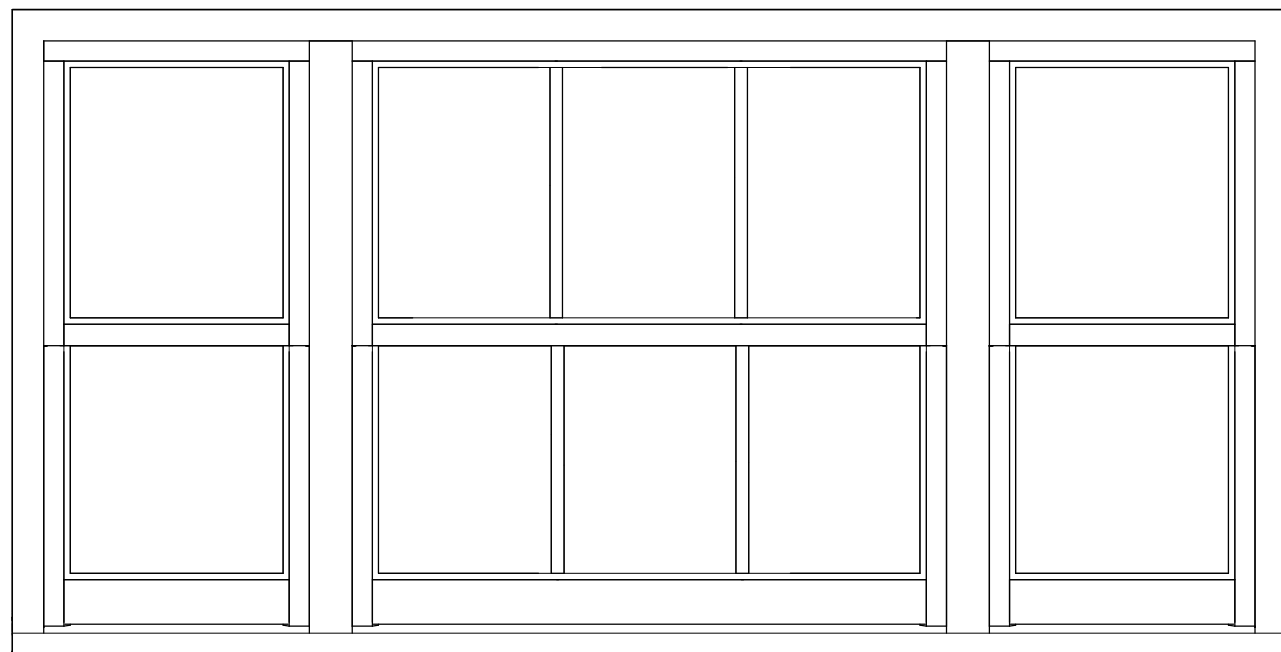
02 Front View 1 : 12
